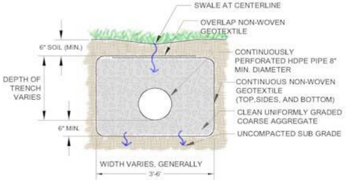
Figure 2: Infiltration Trench Diagram
