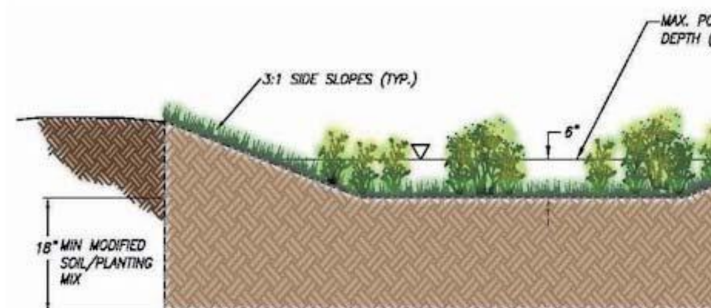
Figure 4: Rain Garden Diagram
