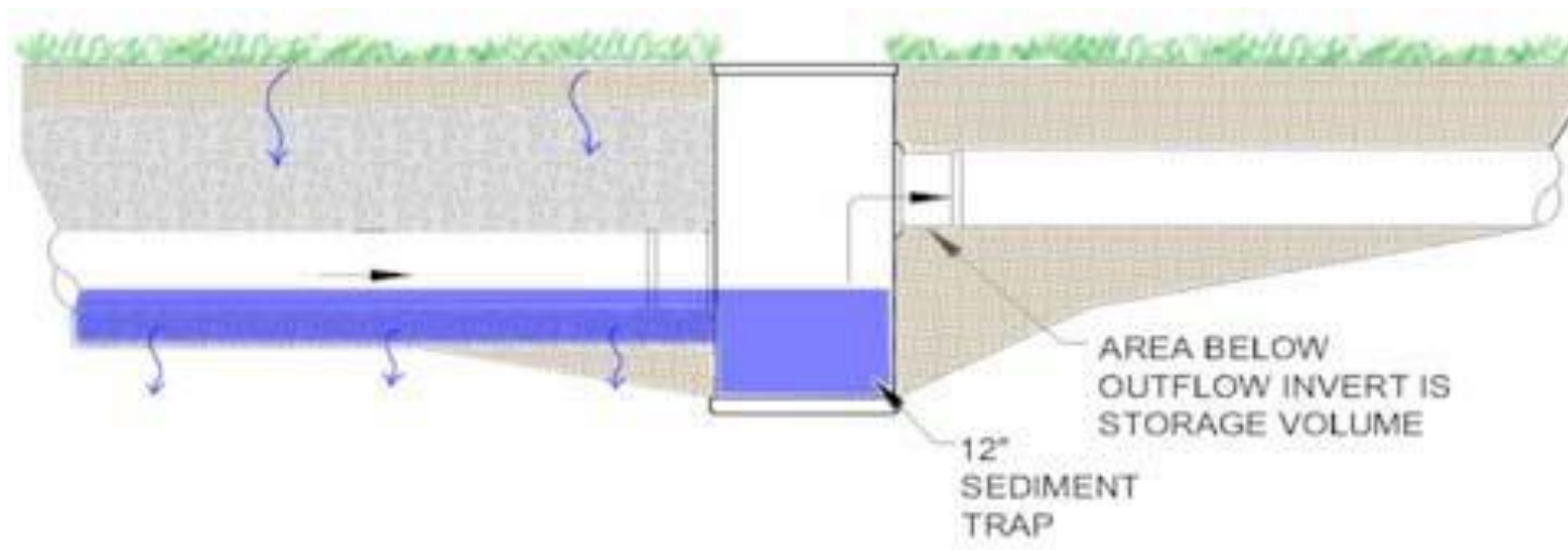
Figure 3: Example of Infiltration Trench Installation
